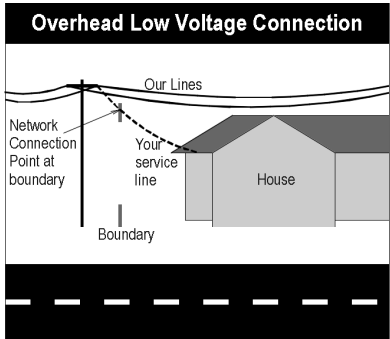
Figure 1 Overhead electricity supply. The Network Connection Point is at the premises boundary.
