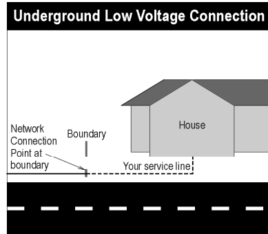
Figure 2 Underground electricity supply. The Network Connection Point is either at the fuse in the servicebox if the servicebox is on the boundary, or on the boundary if the servicebox or pole is not on the boundary.
